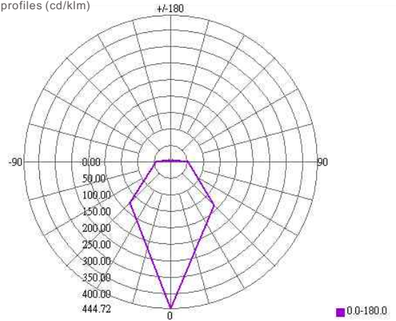
Vertical profiles (cd/klm)
