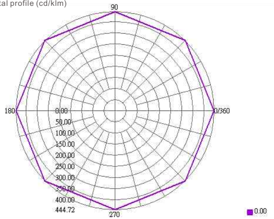
Horizontal profile (cd/klm)
