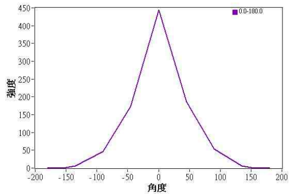
Cartesian coordinates (cd/klm)
